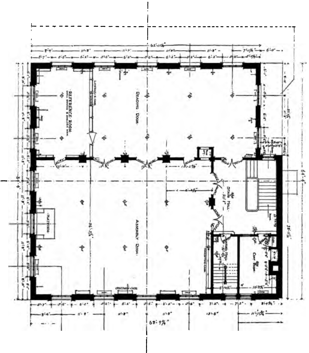
SECOND FLOOR PLAN. TREMONT BRANCH, NEW YORK PUBLIC LIBRARY.
