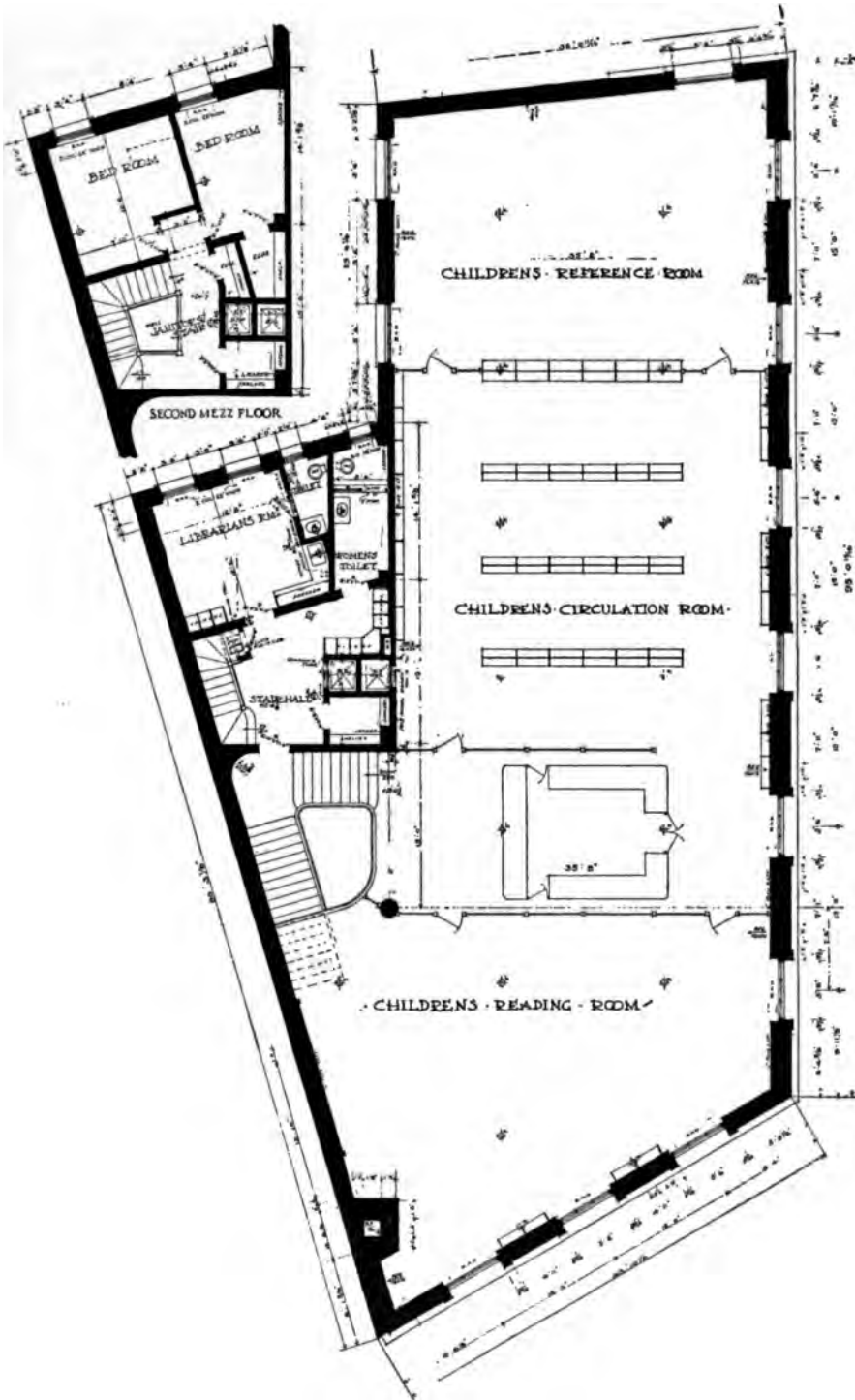
SECOND FLOOR PLAN. HUDSON PARK BRANCH, NEW YORK PUBLIC LIBRARY.
