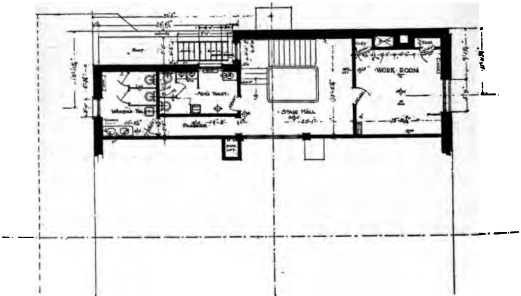
FIRST FLOOR—MEZZANINE—SECOND FLOOR. TREMONT BRANCH, NEW YORK PUBLIC LIBRARY.
