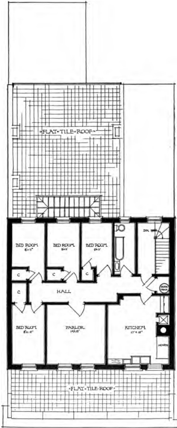
JANITOR'S FLOOR PLAN. RIVINGTON STREET BRANCH, NEW YORK PUBLIC LIBRARY.
