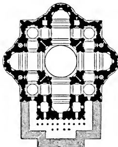
MICHELANGELO GROUND-PLANS OF ST. PETER'S
