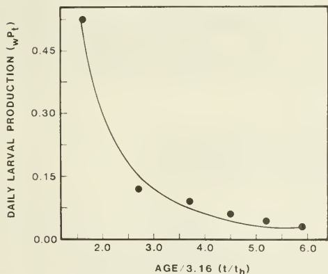
FIGURE 2.—Weighted daily larval production ( {}_wP_t ) and age in days ( t ) of northern anchovy and the fitted larval mortality curve based upon Equation (8B) for larvae < 20 d old, 1979.
