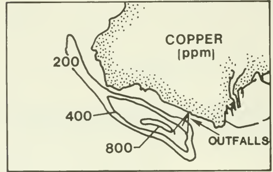
FIGURE 7.—Contour maps of total DDT (ppm dry weight) and copper (ppm dry weight) concentrations in surface sediments on the Palos Verdes shelf in 1975. Maps redrawn from Herselman et al. (1977).
