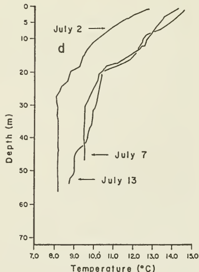
FIGURE 2.—Salinity and temperature profiles during the collections. a. Salinity profiles during the spring collections. b. Spring temperature profiles. c. Summer salinity profiles. d. Summer temperature profiles.
