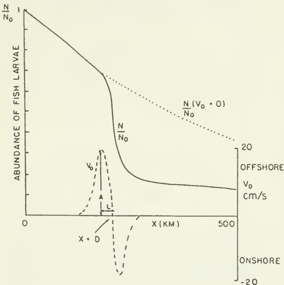
FIGURE 5. - Same as Figure 3 except biological losses ( \mu = 10^{-7} s -1 ) are included.
