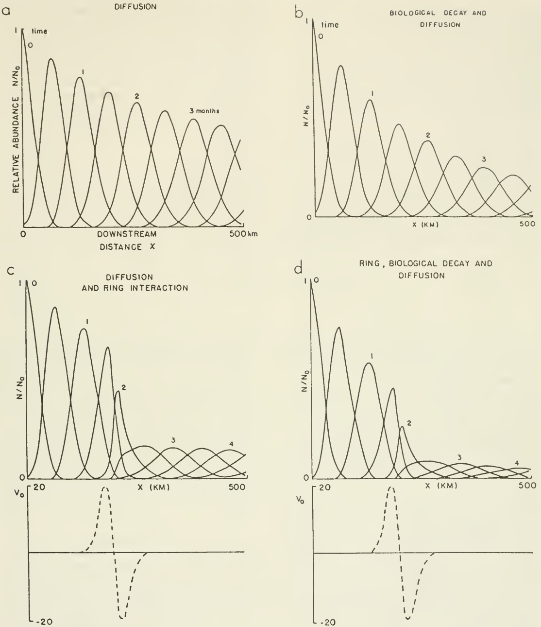
FIGURE 8. - Time-dependent solution of the numerical model which includes a) the diffusion of a spawning group or cohort of larvae as the patch is advected down the shelf. Snapshots are at 15-d intervals. Parameters \mu = 0 , U_0 = 5 cm/s, \Delta x = 5 km, and \Delta t = 0.5 d. b) Same as (a) except \mu = 10^{-7} \text{ s}^{-1} . c) Same as (a) except a stationary ring is present at the shelf edge, with parameters A = 20 cm/s and L = 20 km. d) Same as (c) except \mu = 10^{-7} \text{ s}^{-1} .
