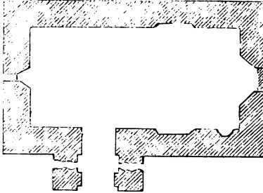
Ground-plan of St. Michael's Chapel, at Torr.
