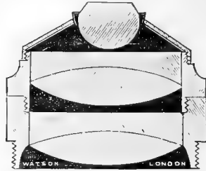
Fig. 69.—Achromatic Condenser. This is specially designed for use in photo-micrography, but it is also efficient for visual work. It does the work of the Abbe Illuminator, and transmits a rather larger aplanatic cone of light. It is strongly recommended where critical photographic work is to be done. It may be used with the highest power objectives, and by removing the top lens can be used with the lowest powers. The new Schott glass is employed in its construction.
