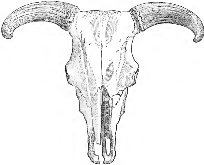
Skull of Dos primigenius , found at Mugdrum, 27 \frac{3}{4} inches in length. See p. 2.
