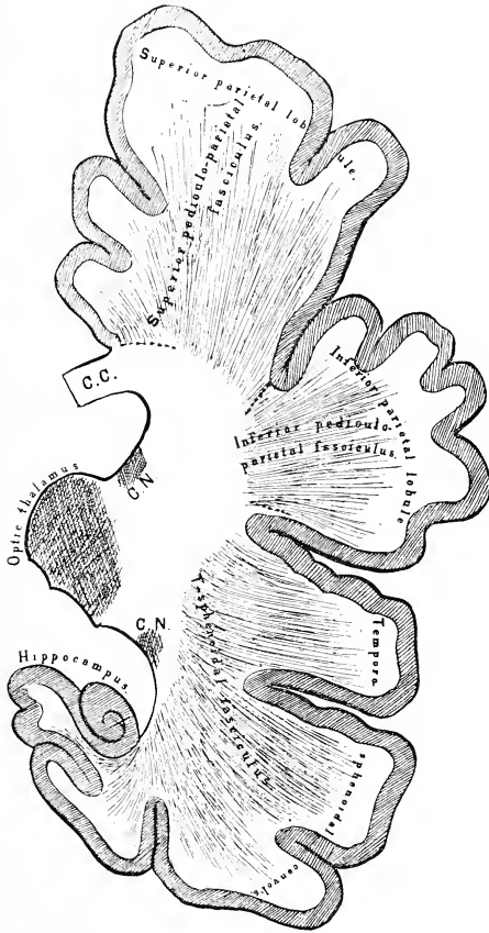
№7. PEDICULO-PARIETAL SECTION
